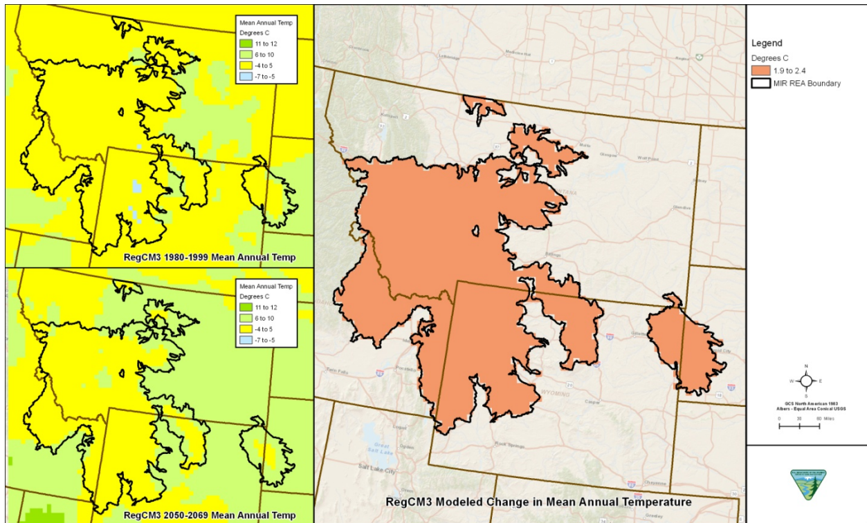
Figure 6-4. Current (1980-1999) and Future (2050-2069) Mean Annual Temperatures
