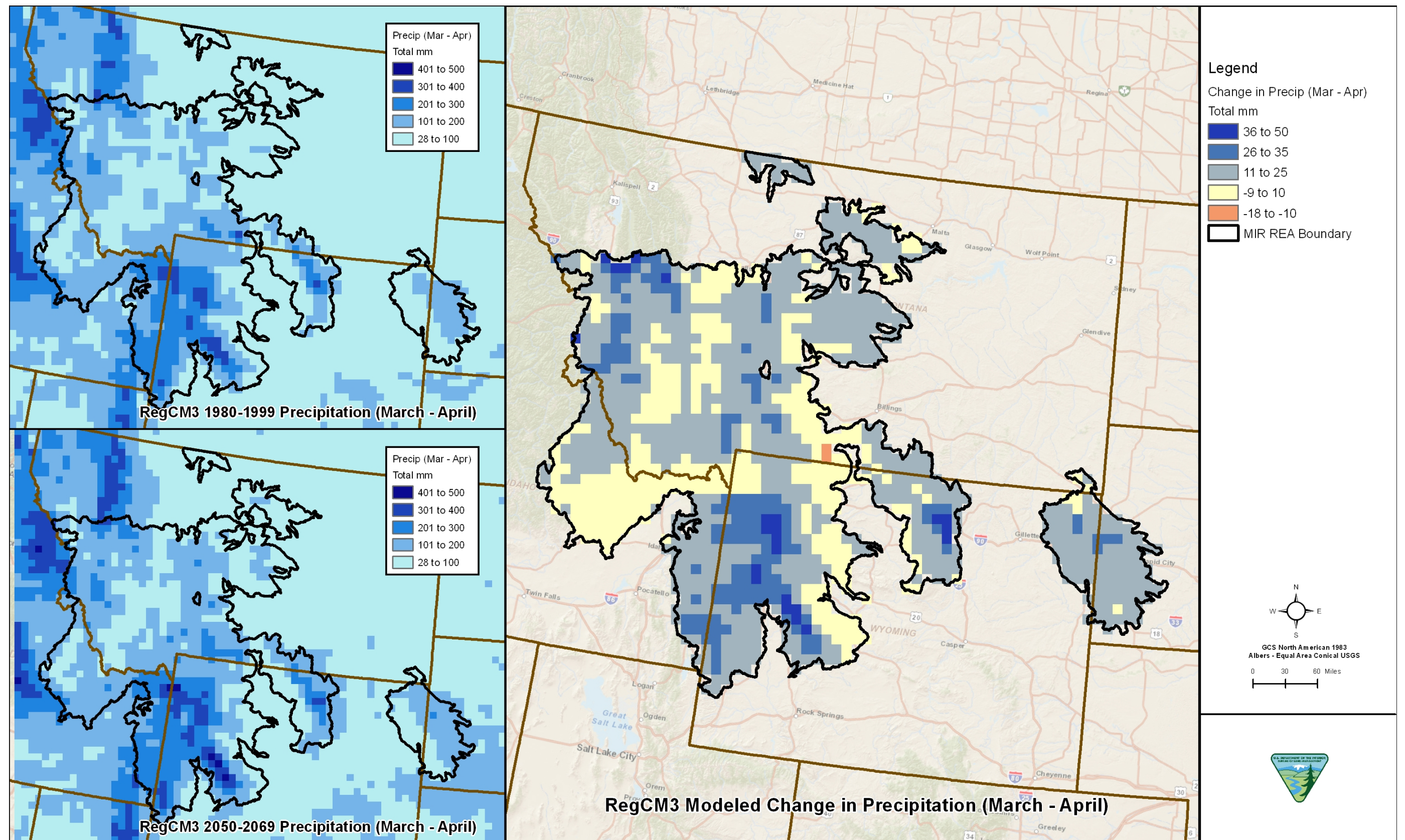
Figure C-5-2. Precipitation March and April
