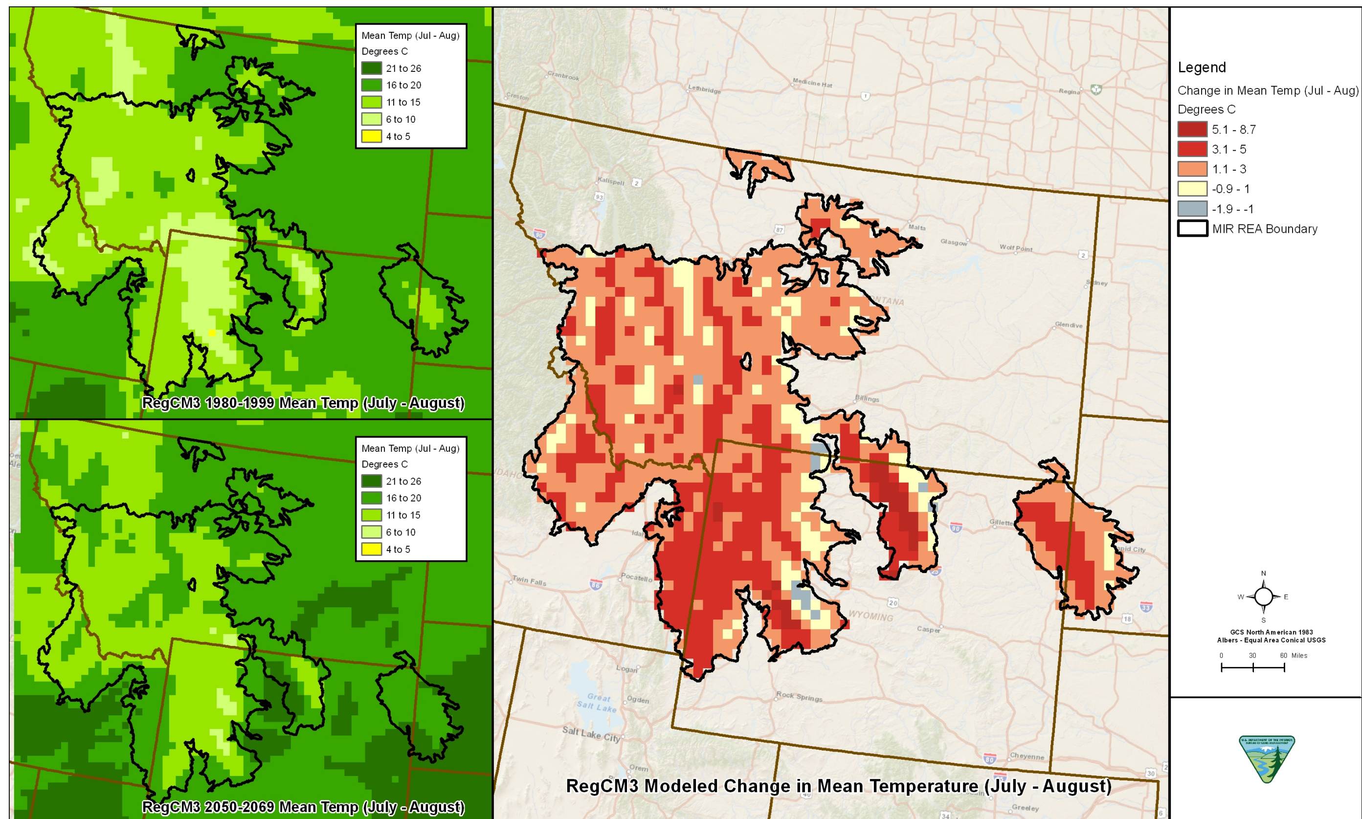
Figure C-5-11. Temperature July and August
