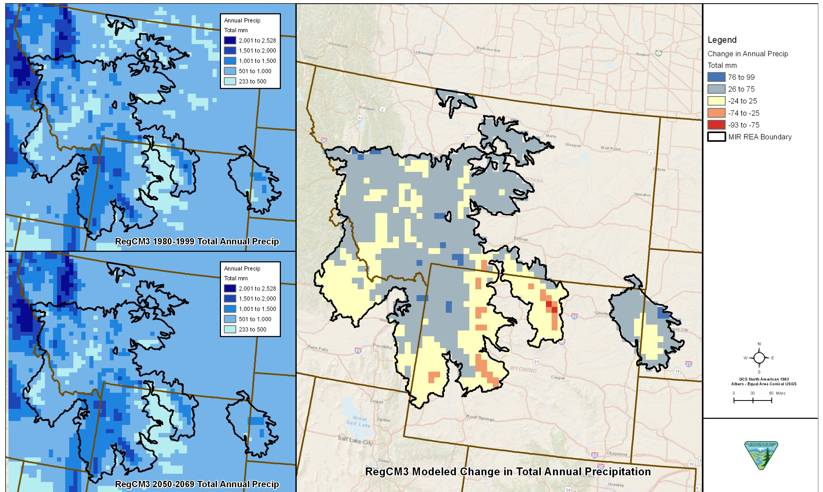
Figure C-5-1. Annual Precipitation
