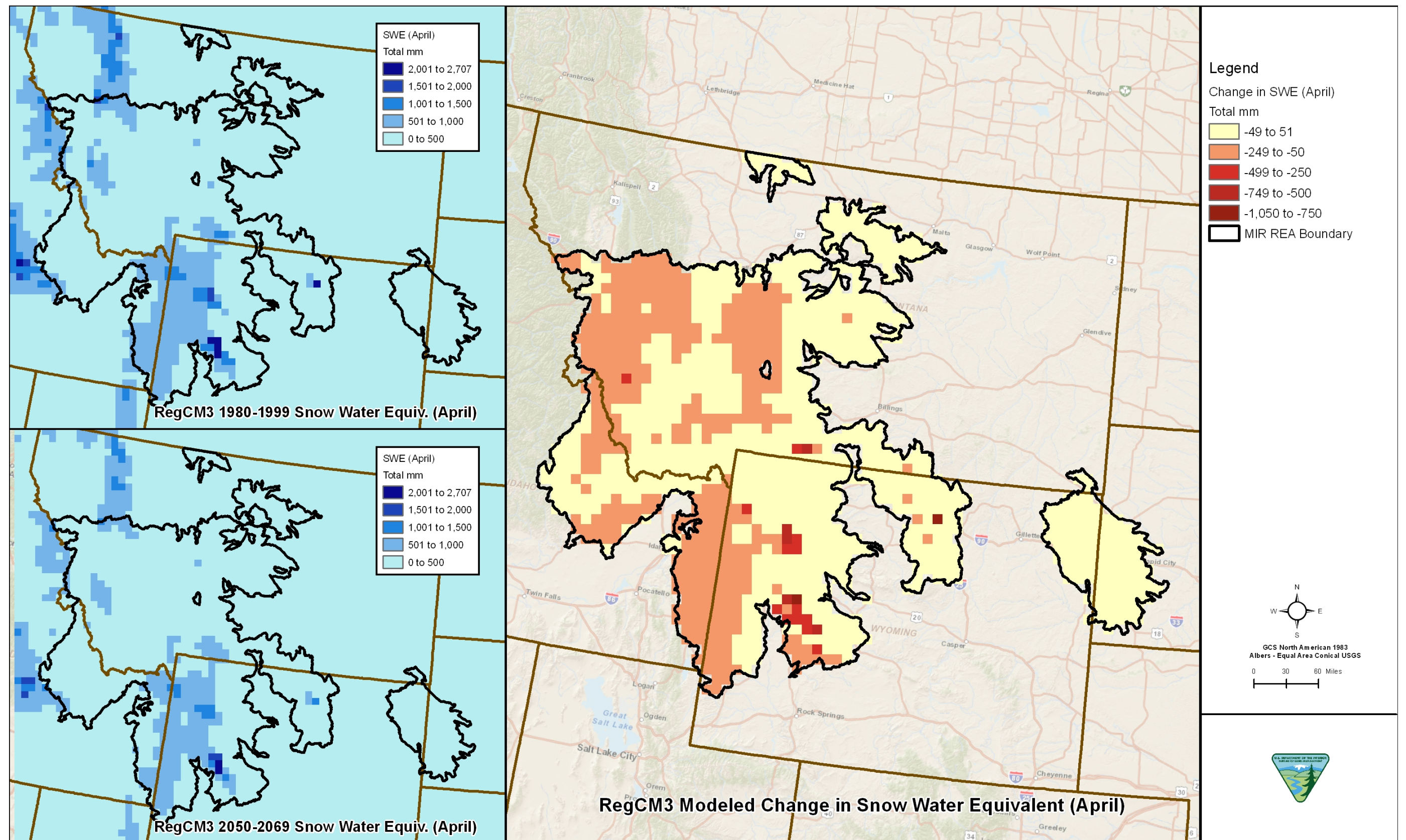
Figure C-5-7. Snow Water Equivalent (April)
