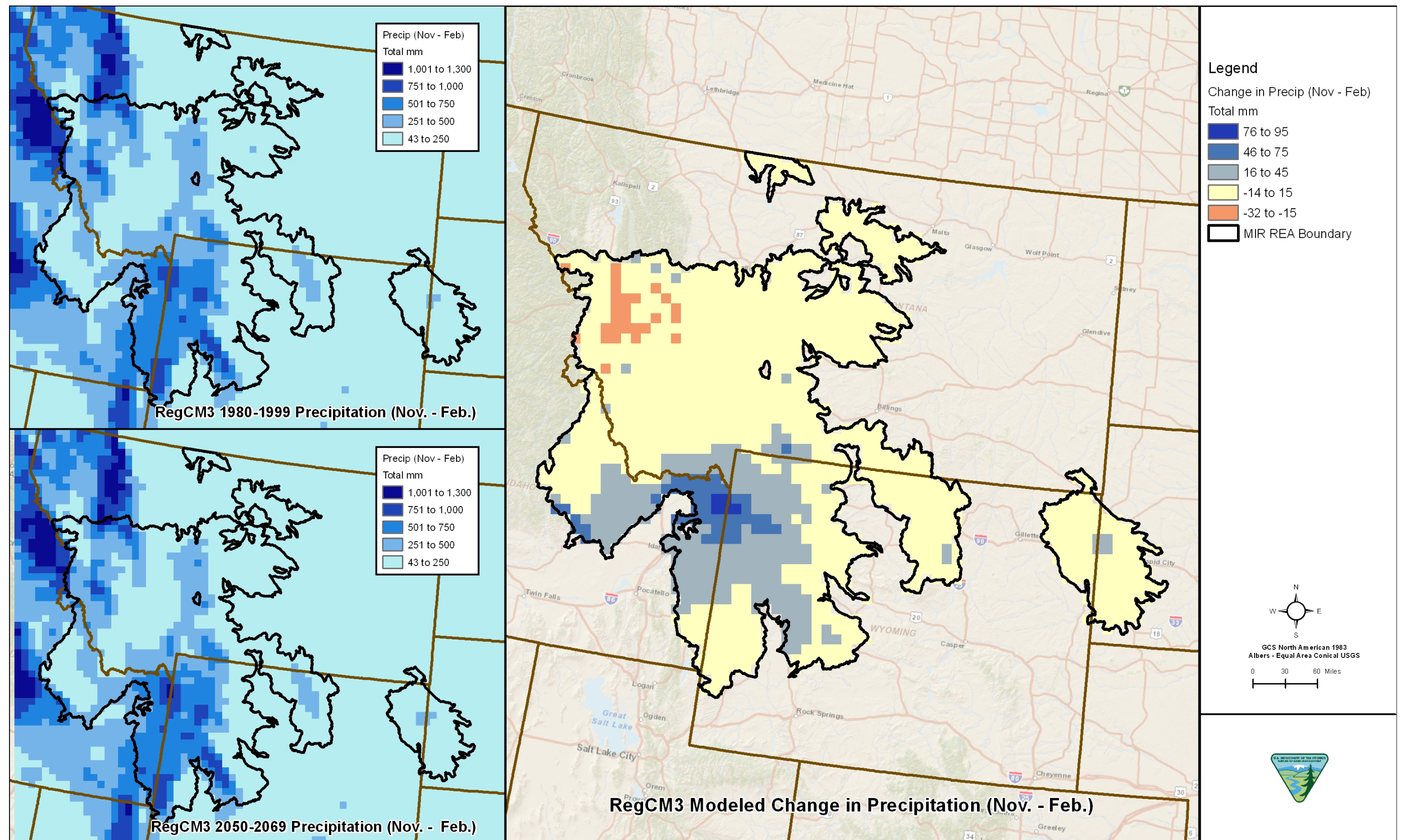
Figure C-5-6. Precipitation November to February
