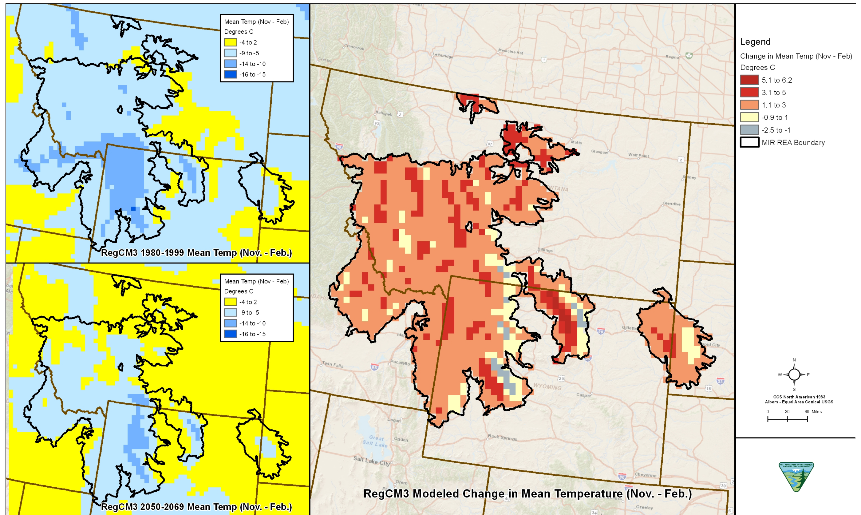
Figure C-5-13. Temperature November to February
