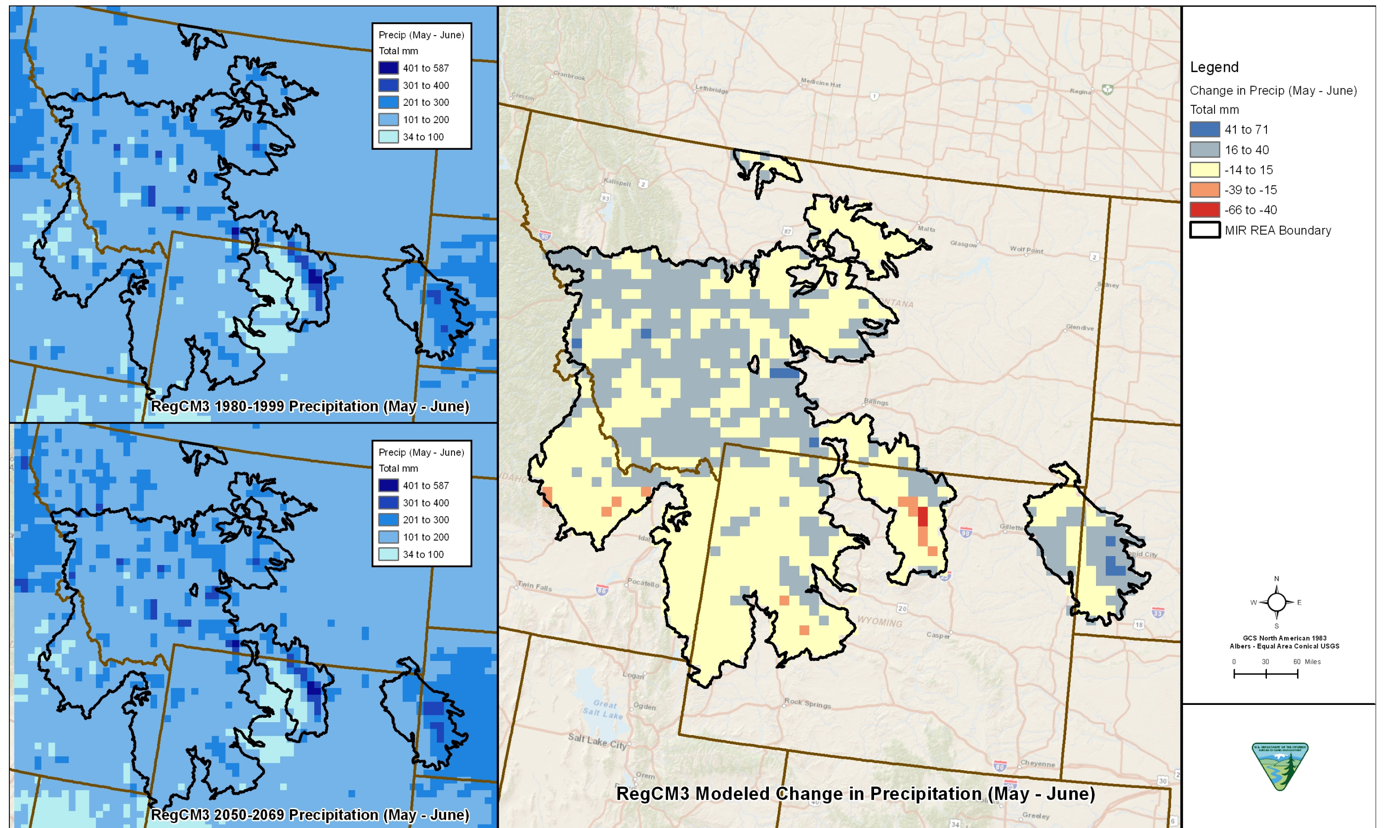
Figure C-5-3. Precipitation May and June
