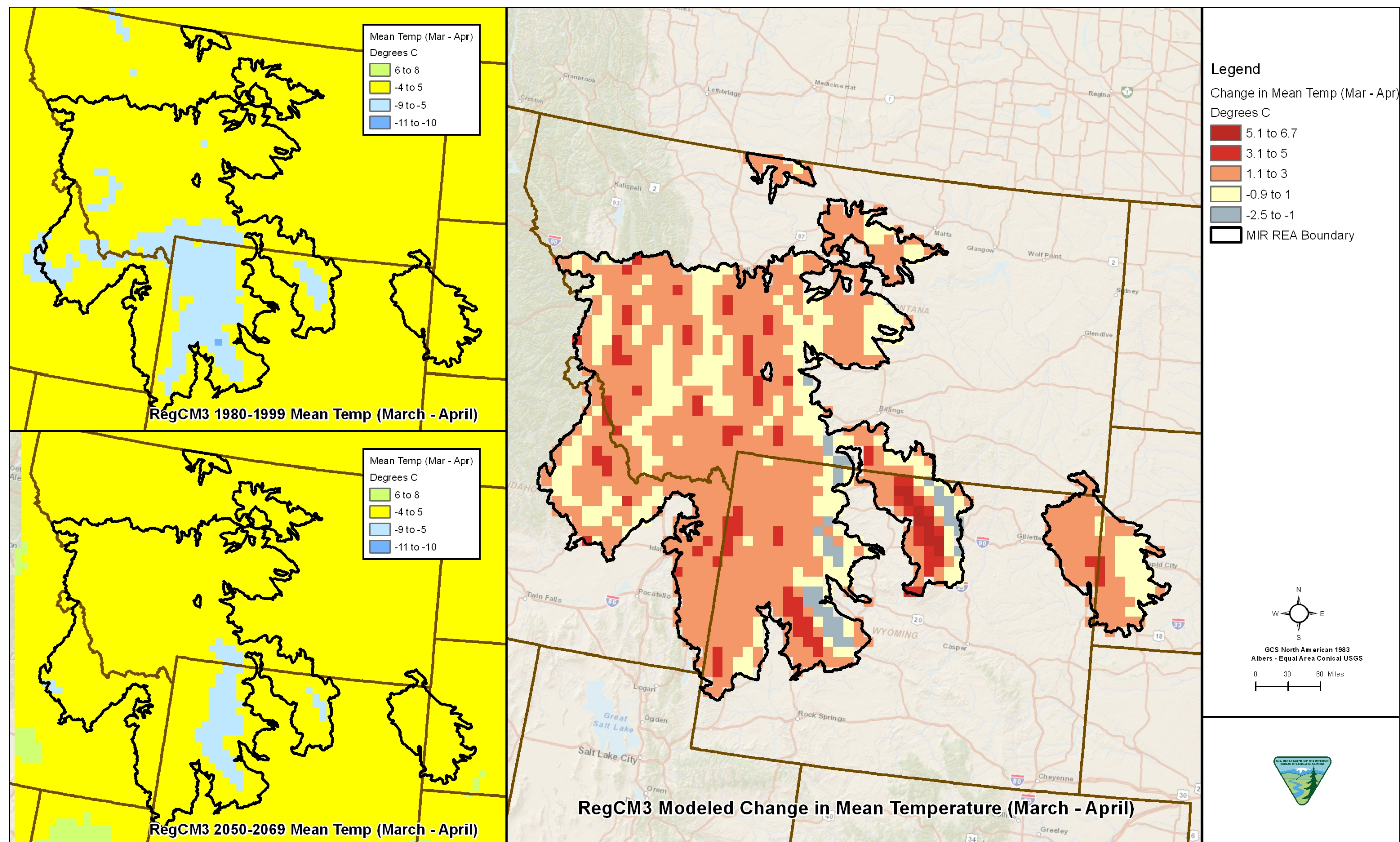
Figure C-5-9. Temperature March and April
