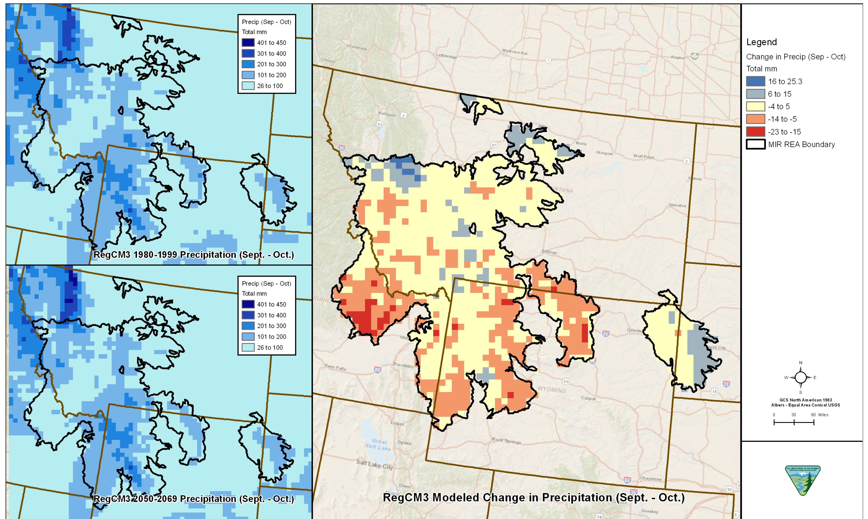
Figure C-5-5. Precipitation September to October
