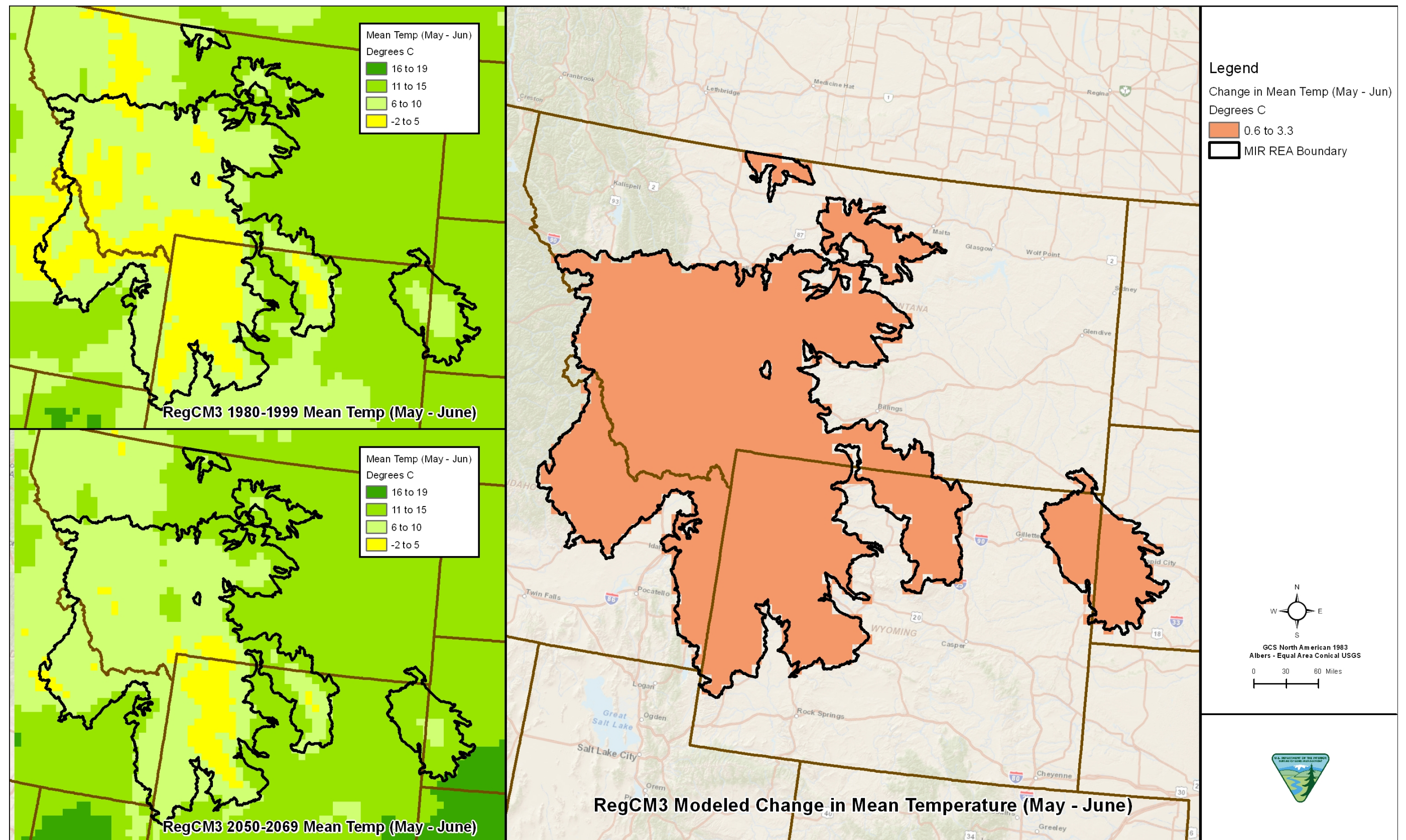
Figure C-5-10. Temperature May and June
