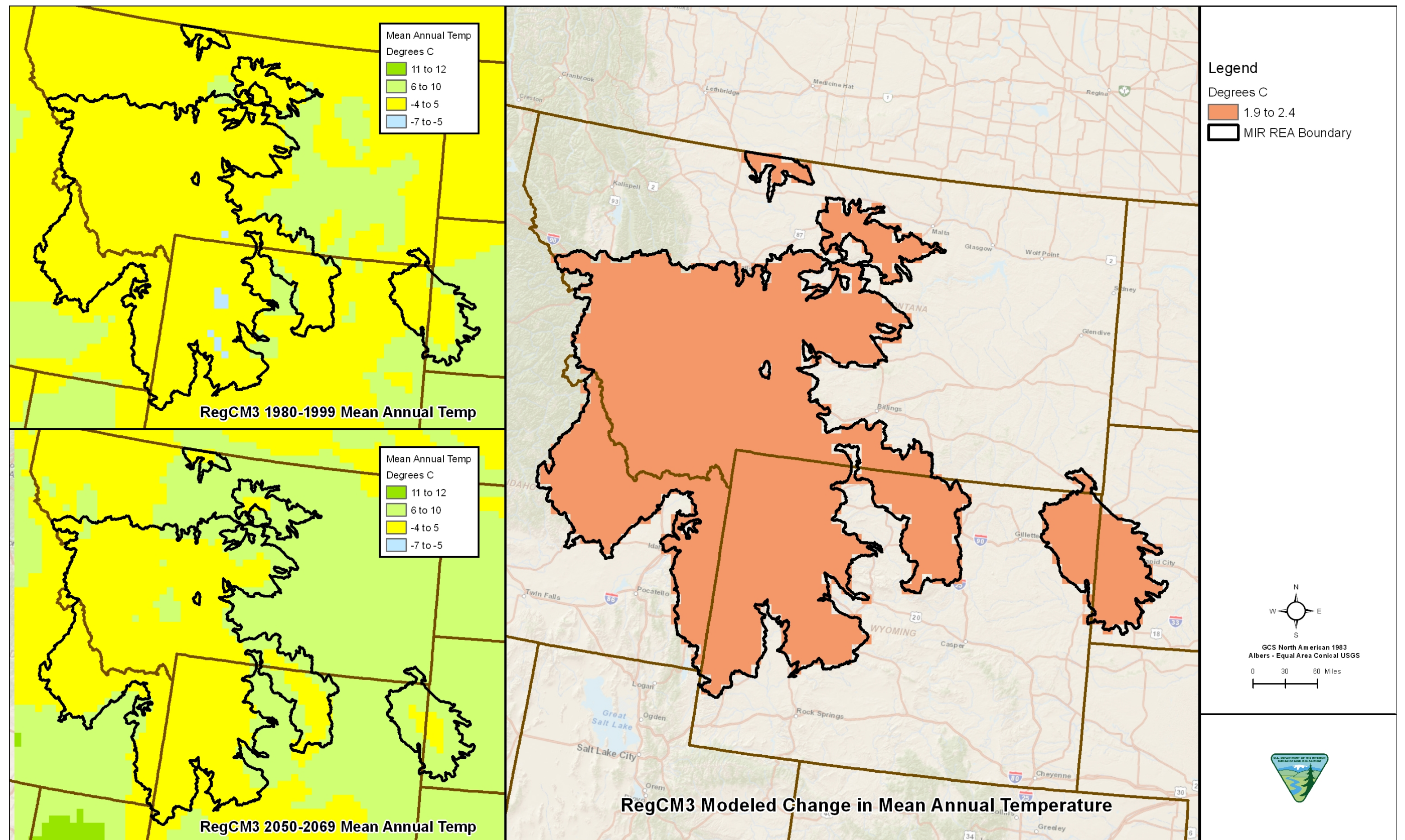
Figure C-5-8. Annual Temperature
