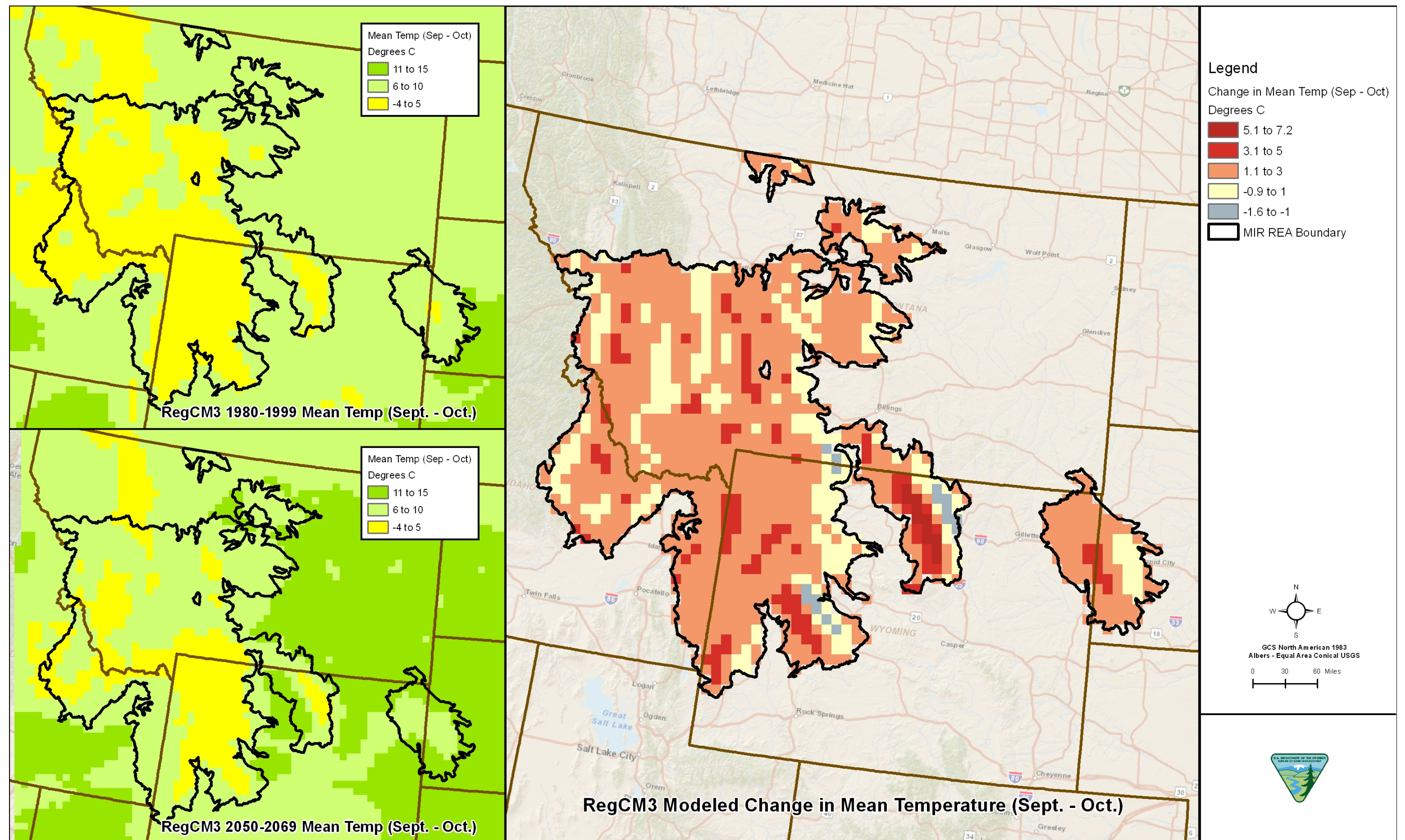
Figure C-5-12. Temperature September to October
