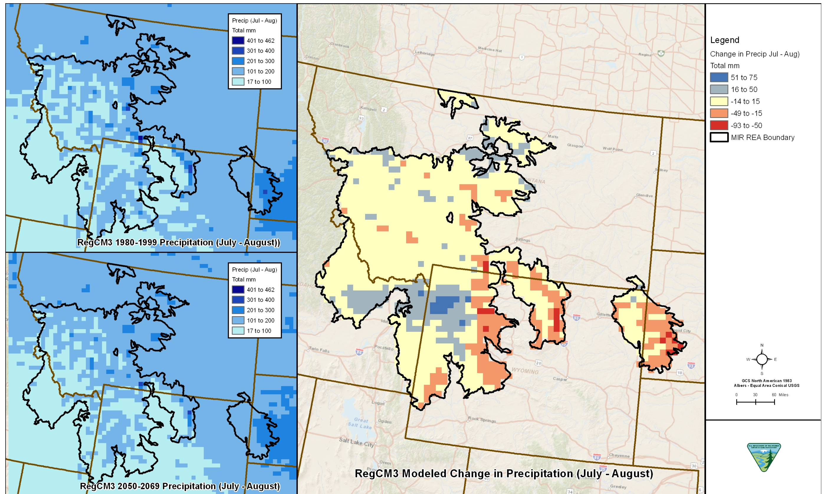
Figure C-5-4. Precipitation July and August
