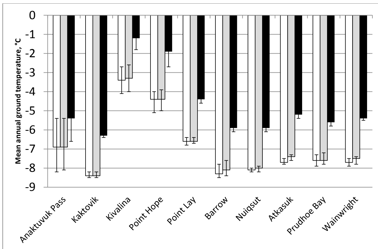
Figure C-30. Mean annual ground temperature (°C) at one meter depth (MAGT) for community watersheds in the North Slope study area. Current (white), near-term (light gray), and long-term (dark gray) time steps are shown. Active layer thickness is expected to increase across the North Slope study area (Figure C-31). Figure C-32 demonstrates the high ALT variability by sub-region, as well as within each sub-region. Maximum and minimum values are shown by error bars.
